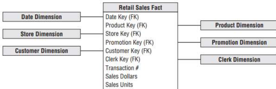
Fig. 3. Star schema in the retail sales fact table
