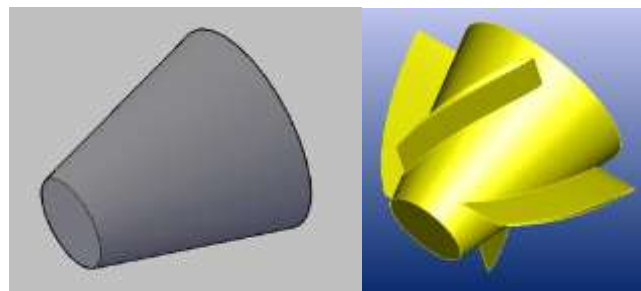
Fig. 5 PBCF Hub and PBCF with 70° Pitch angle
